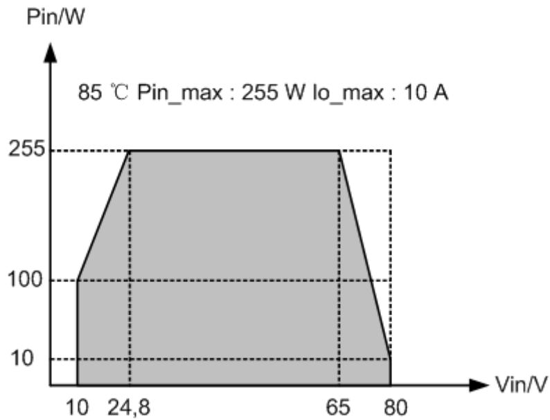
Figure A-6 Courbe de relation P_{in} - V_{in} ( 85^\circ\text{C} , P_{in\_max} = 255\text{ W} , I_{o\_max} = 10\text{ A} )
