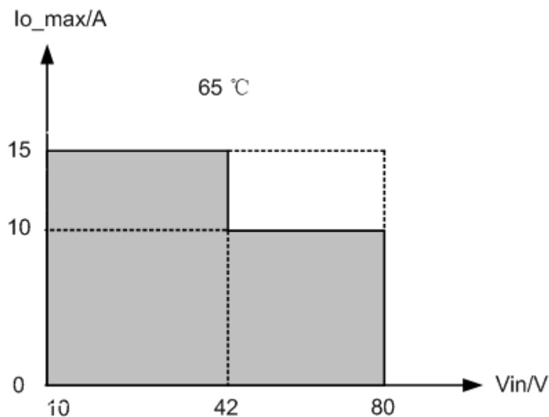
Figure A-2 Courbe de relation I_{o\_max} - V_{in} (65°C)
